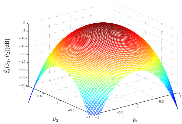
(b) The case of Gaussian autocorrelation function
