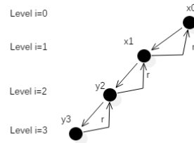
Flow graphs modeling Algorithm 1.4
