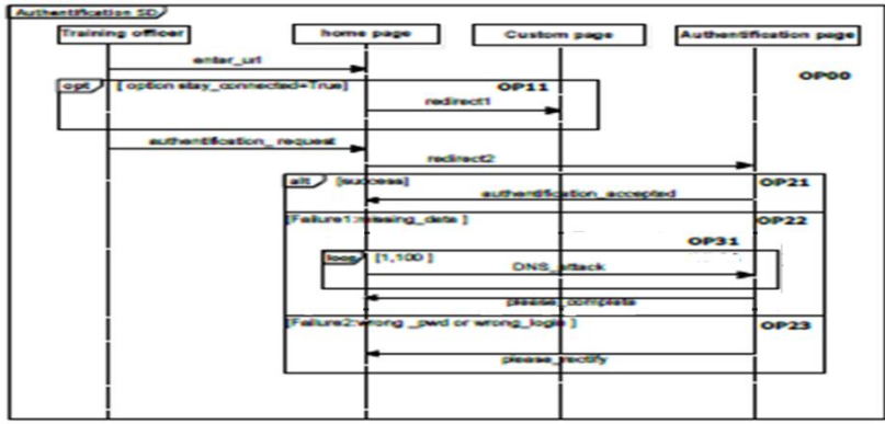
Fig. 1. Authentication SD
