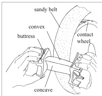
Fig. 18. Manual polishing of aero engine turbine vanes
