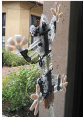
Fig. 16. Stickbot http://bdml.stanford.edu/twiki/bin/view/Main/StickyBot
