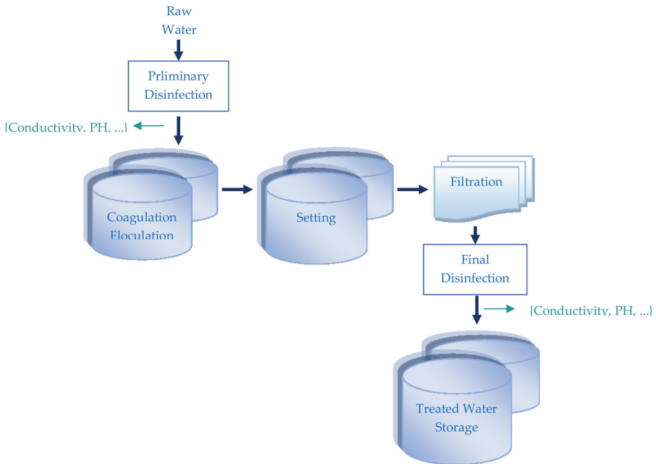
Figure 1. Simplified synopsis of the water treatment plant.
