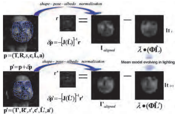
Fig. 7. Two consecutive iterations of the fitting process. During the iteration It_i a region in the test image is captured and normalized according to the current parameters p producing the image I_{aligned} . A residual r is calculated by comparing I_{aligned} with a reference shape-normalized model illuminated by the current parameter \hat{L} . An additive increment vector \delta p is computed. \delta p is iteratively reduced by re-scaling it (step 15) until the energy of the residual is lower than its initial estimate. When this event occurs, the new set of model parameters p' is used again to normalize a new region within the test image. The new residual r' in combination with a new Jacobian J(\hat{L}') is used to compute a new set of increments to the parameters, and so on.
