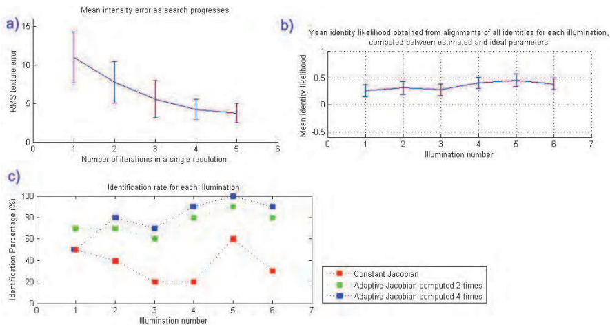
Fig. 10. a) Evolution of RMS error in intensity difference. b) Average (over the 10 identities) of the identity likelihood measured between estimated and ideal parameters. c) Identification rates for each one of the six illuminations.
