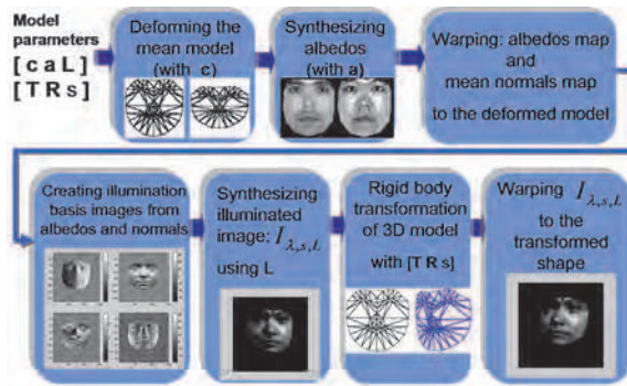
Fig. 4. Face synthesis process.
