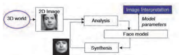
Fig. 1. Schematized flow of the analysis by synthesis approach.
