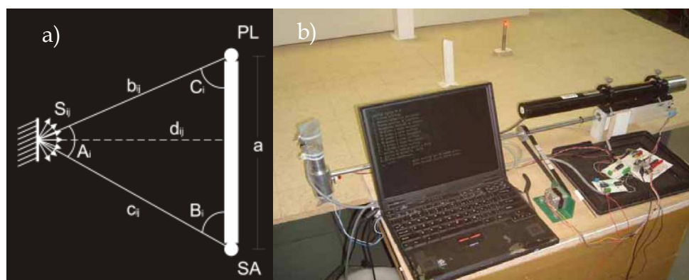
Fig. 10. a) Triangulation scheme, b) Dynamic triangulation scanner
