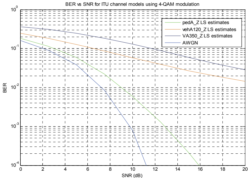
Fig. 6. BER performance of LTE transceiver for different channel models using QPSK modulation and LS channel estimation
