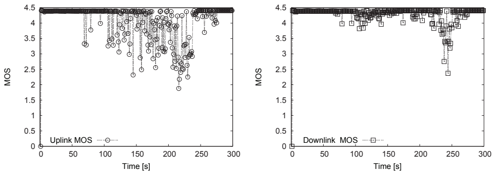
Fig. 30. MOS during movement (from WiMAX to WLAN)
