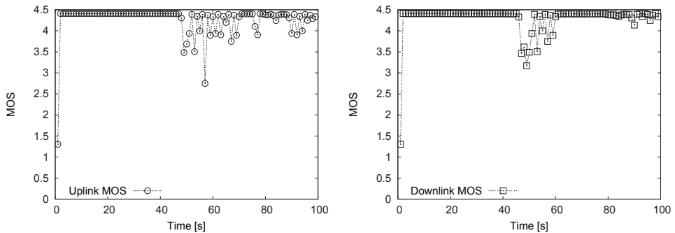
Fig. 31. MOS over congested wireless network (WLAN)
