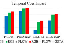
Figure 7: Temporal impact.
