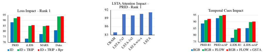
Figure 5: Loss impact.
