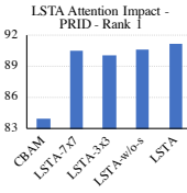
Figure 6: Attention impact.
