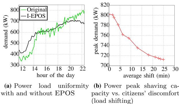
Fig. 17 Load balancing of power demand with EPOS [96]
