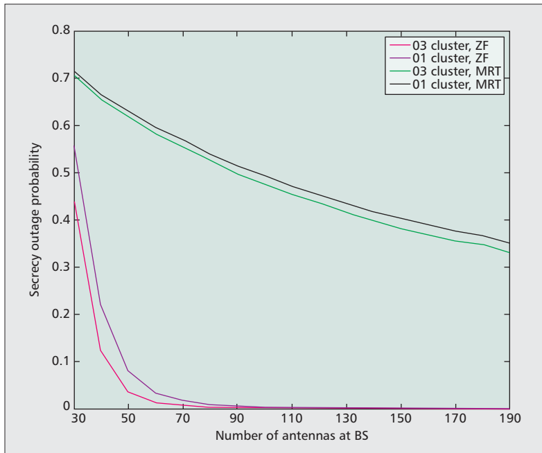
Figure 4. The secrecy outage probability of downlink with MRT and ZF precoding techniques at the BS. We consider three hexagonal cells without sectorization, where the radius of each cell is 350 meters. In each cell, seven single-antenna users are uniformly distributed and one of them is an eavesdropper. In this figure “01 cluster” means that the frequency reuse pattern is 1 while “03 cluster” means that the frequency reuse pattern is 3.
