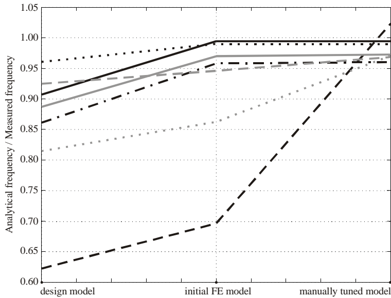
Figure 6: Manual frequency tuning of different FE models (1HS – solid black line; 1VS – dotted black line; 1VA – dashed black line; 1HA – dot-dashed black line; 2HS – solid grey line; 2VA – dotted grey line; 2VS – dashed grey line).
