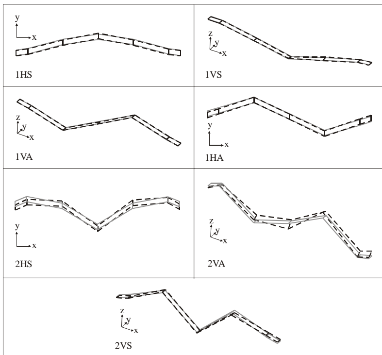
Figure 11: Overlaying of mode shapes obtained experimentally (black dashed line) and numerically in the final FE model (grey line).
