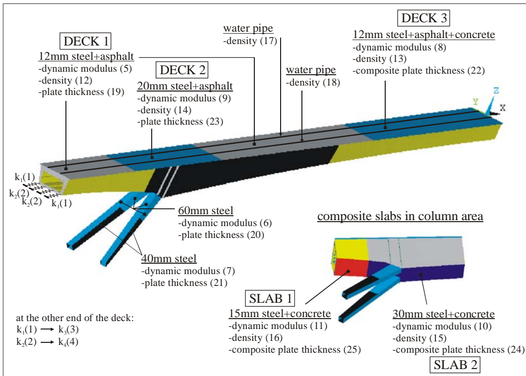
Figure 7: Uncertain parameters in the manually tuned FE model.
