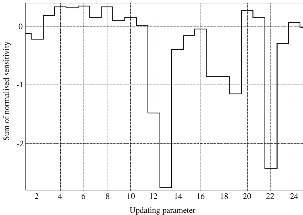
Figure 8: Plot of sum of normalised sensitivity of 14 selected target responses to 25 uncertain parameters in the manually tuned FE model.
