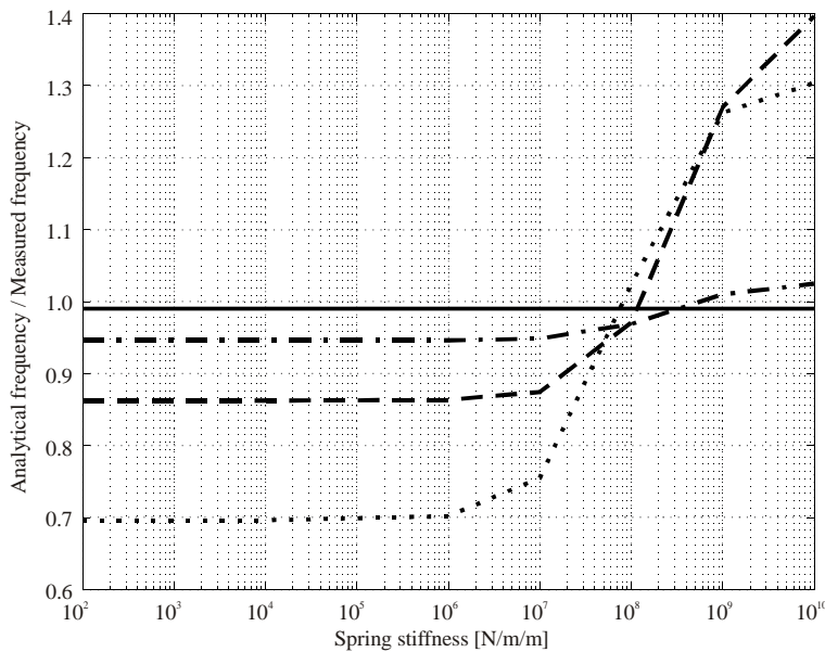
Figure 5: Choice of appropriate stiffness for spring supports at the ends of the box girder (1VS – solid line; 1VA – dotted line; 2VA – dashed line; 2VS – dot-dashed line).
