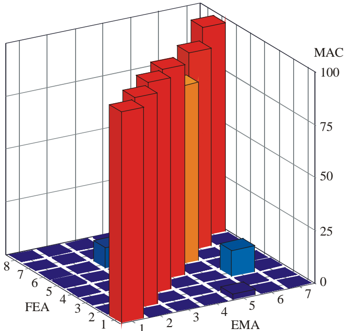
Figure 10: MAC matrix after updating. FEA and EMA stand for FE model and experimental model, respectively.
