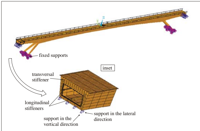
Figure 3: Initial FE model.
