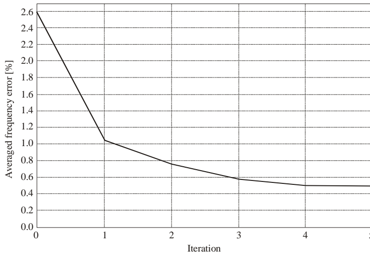
Figure 9: Convergence of the iterative process presented via averaged frequency error.
