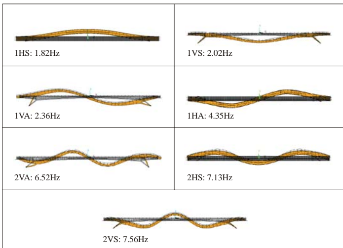
Figure 4: Modes of vibration calculated from the initial FE model.
