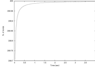
Figure 2. Time-evolution of bonds density.
