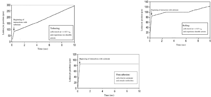
Figure 3. Representative trajectory of lymphocyte tethering at a mean velocity v equal to one half of the hydrodynamic velocity v_h . The parameters are the following: \gamma = 0.001 nm, k_{on} = 84s^{-1} , k_{off}^{(u)} = 1s^{-1} (upper left). Representative trajectory of rolling motion of lymphocyte, with a mean velocity v < 0.5v_h , that experience durable arrests (upper right). Representative trajectory of lymphocyte for firm adhesion. The parameters are the following: \gamma = 0.001nm , k_{on} = 84s^{-1} , k_{off}^{(u)} = 20s^{-1} (lower).
