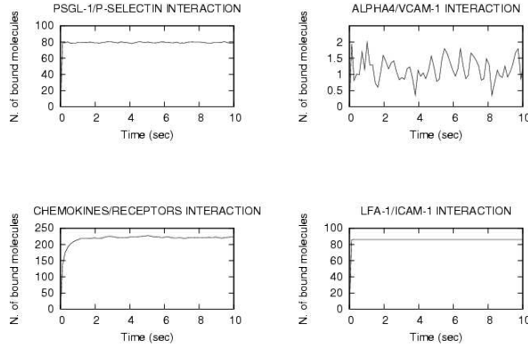
Figure 4. BioSpi simulation of 4-phases model of lymphocyte recruitment.
