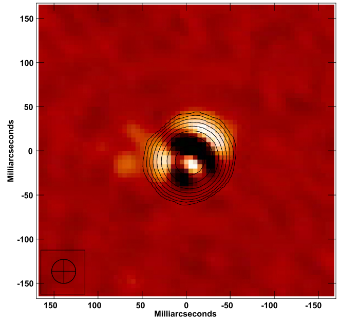
Figure 6. Contour map of the 229 GHz emission from Mira A (reproduced from Figure 3), overplotted on an image of the residuals after subtraction of the best-fitting uniform elliptical disk model. The residuals range from -1.4 to +0.9 mJy beam ^{-1} , with the peak positive residual lying slightly southwest of the nominal disk center. In comparison, the peak surface brightness of the observed stellar emission is 71.1 mJy beam ^{-1} . The restoring beam (FWHM 27.3 mas) is indicated in the lower left corner.
