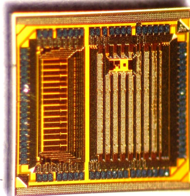
Figure 6. Micrograph of prototype ASIC.
